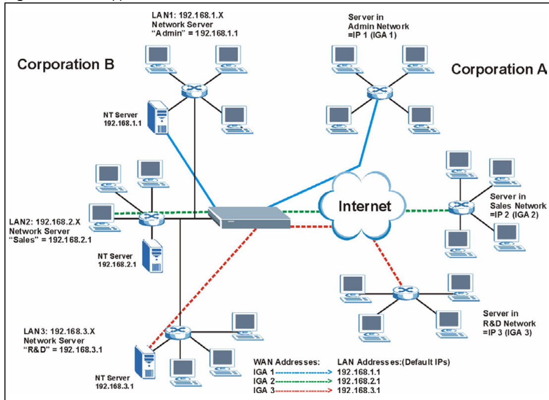
Figure 43 NAT Application With IP Alias
