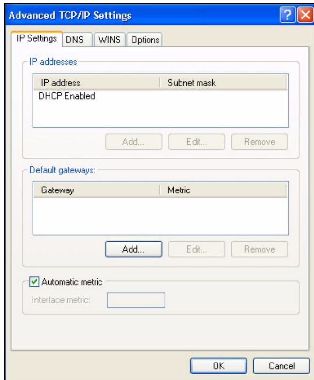
Figure 104 Windows XP: Advanced TCP/IP Properties
