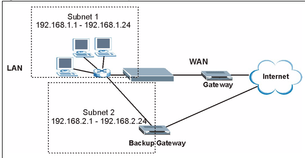
Figure 32 Traffic Redirect LAN Setup
