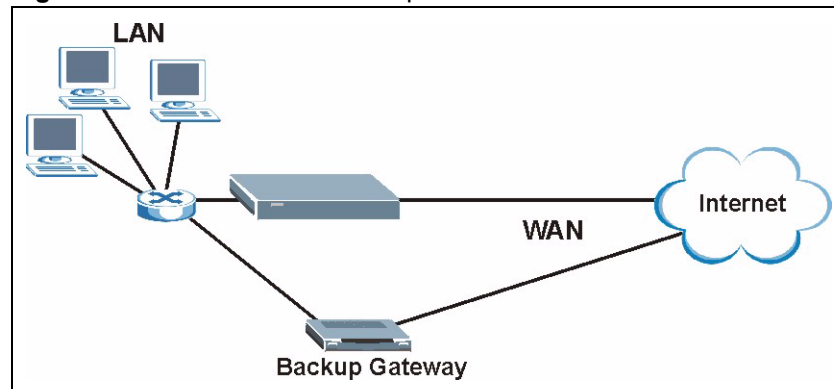
Figure 31 Traffic Redirect Example
