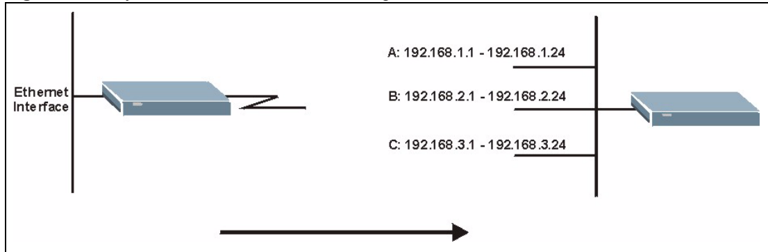
Figure 40 Physical Network & Partitioned Logical Networks
