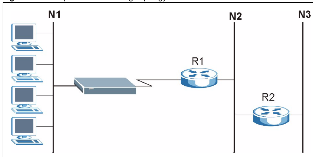
Figure 50 Example of Static Routing Topology
