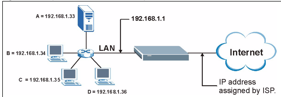
Figure 45 Multiple Servers Behind NAT Example
