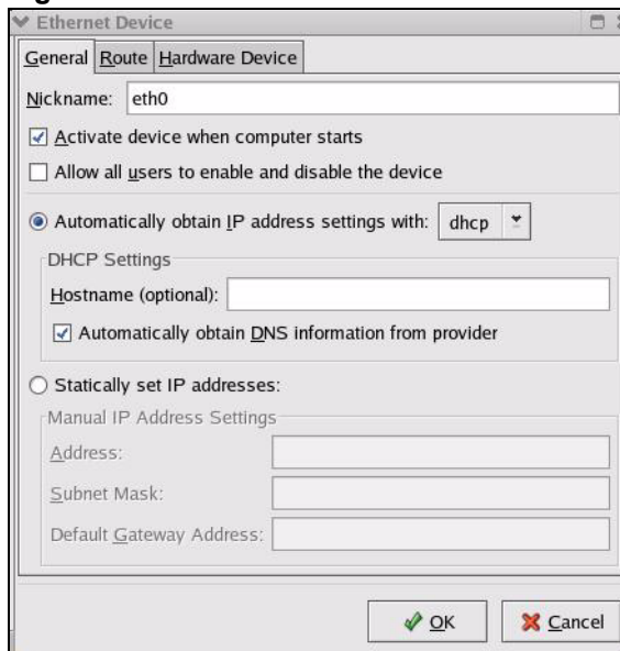
Figure 111 Red Hat 9.0: KDE: Ethernet Device: General
