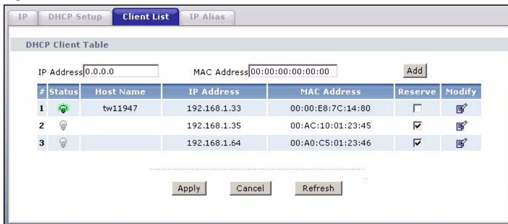
Figure 39 LAN Client List
