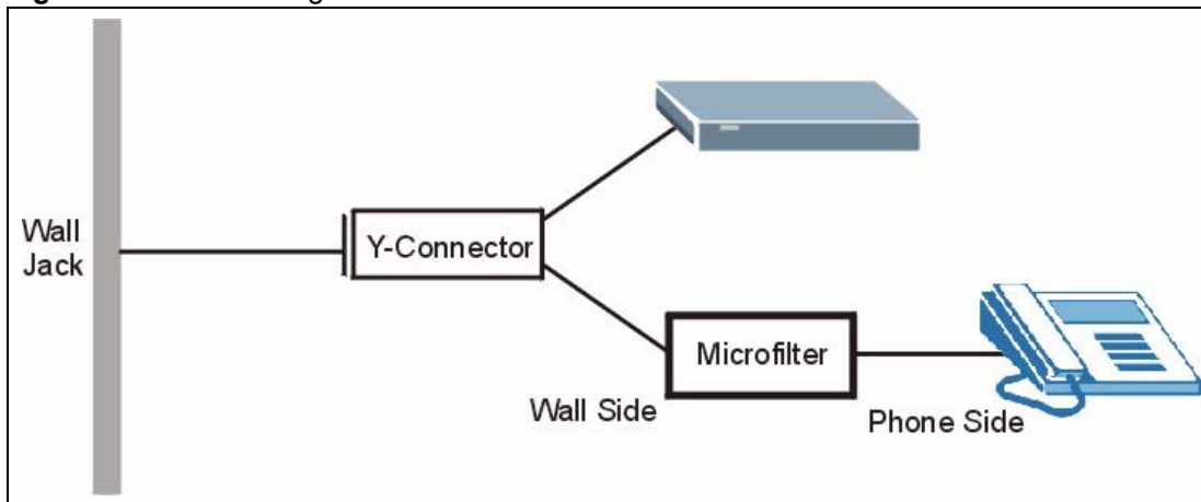
Figure 121 Connecting a Microfilter and Y-Connector
