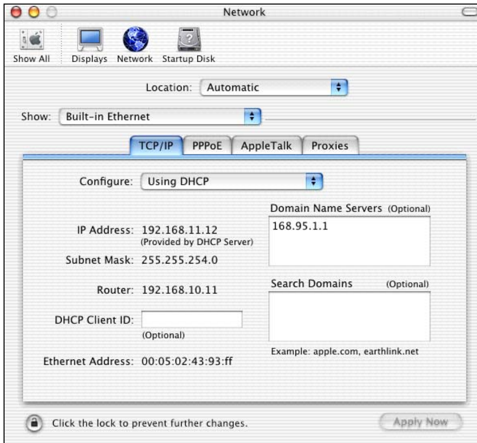
Figure 109 Macintosh OS X: Network
