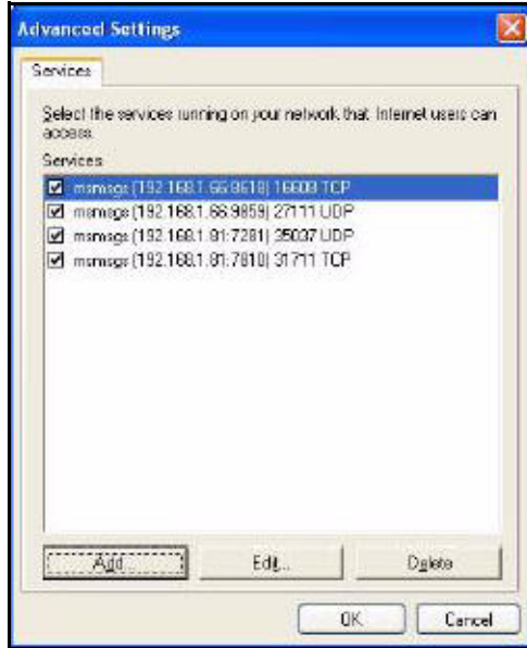
Figure 71 Internet Connection Properties: Advanced Settings: Add
