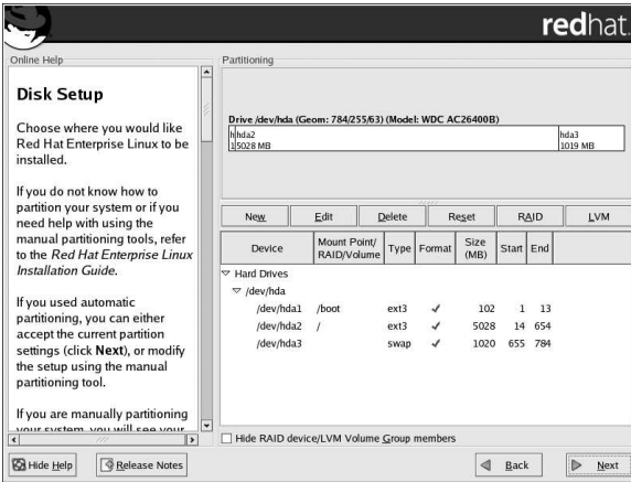
Figure 4-12. Partitioning with Disk Druid on x86, AMD64, and Intel® EM64T Systems
