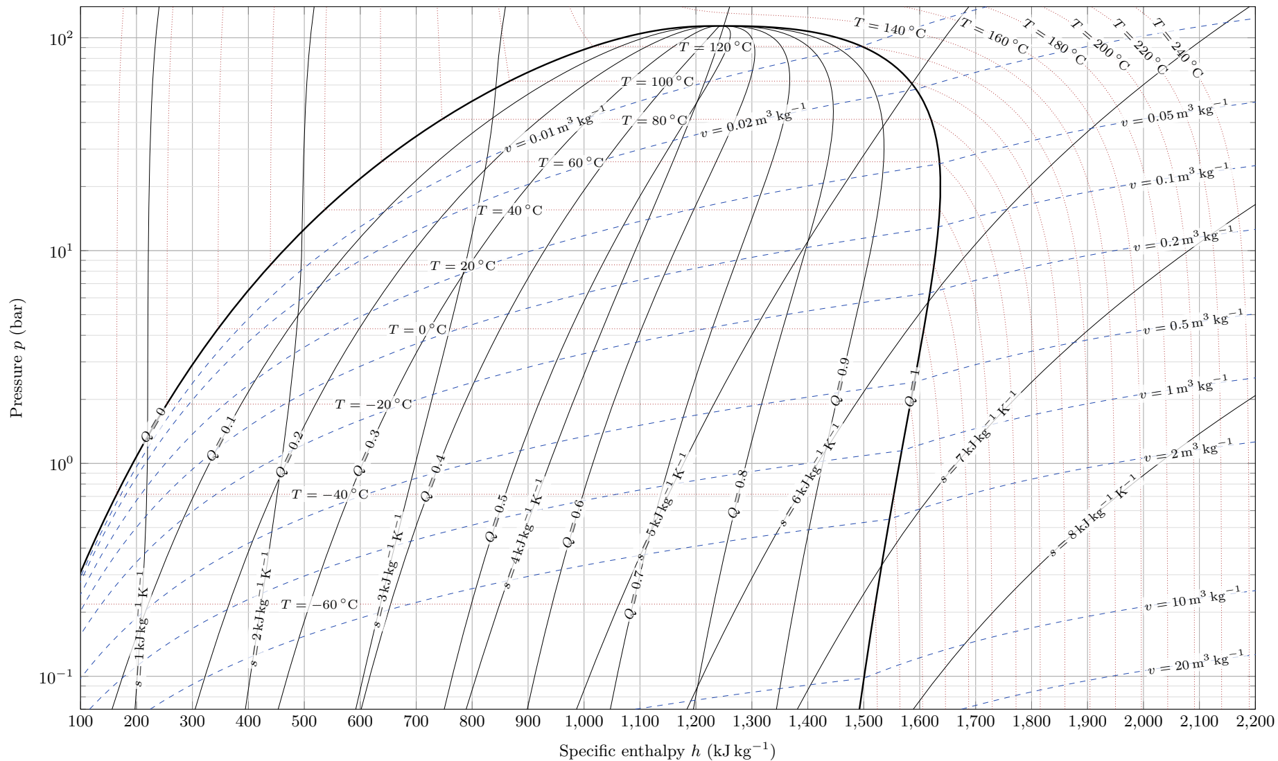
R717 pressure–enthalpy diagram
