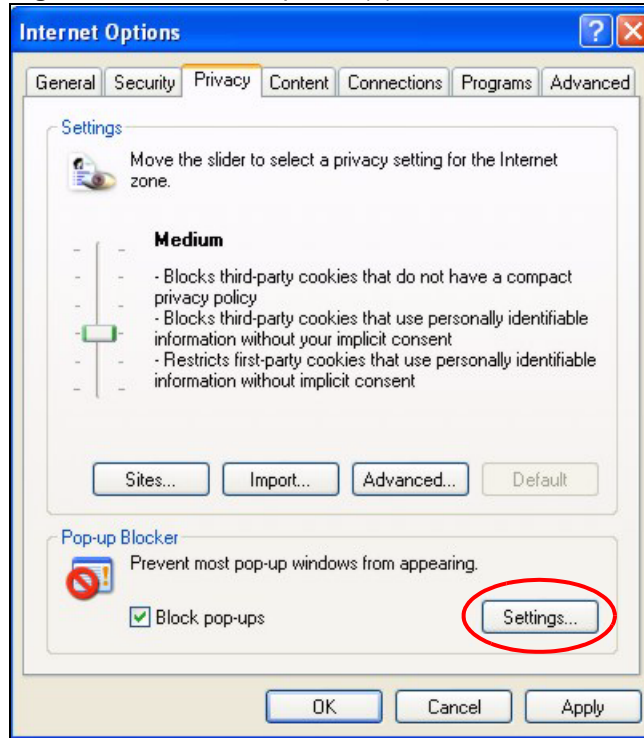
Figure 190 Internet Options (2)
