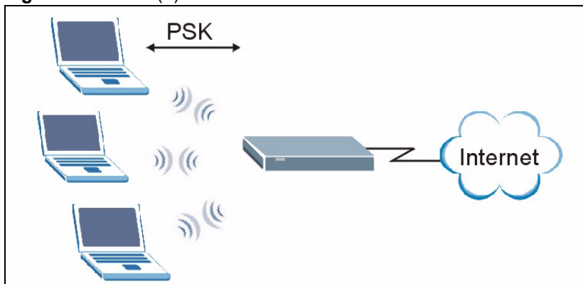
Figure 187 WPA(2)-PSK Authentication
