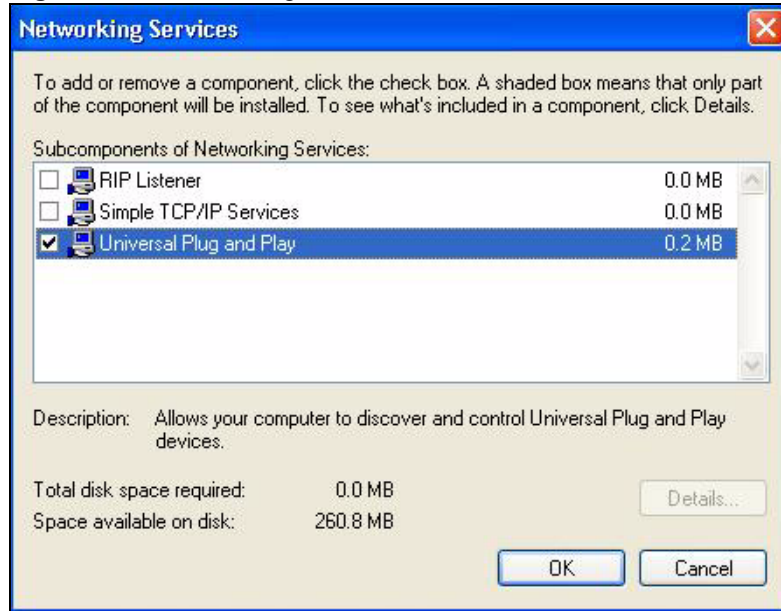
Figure 121 Networking Services
