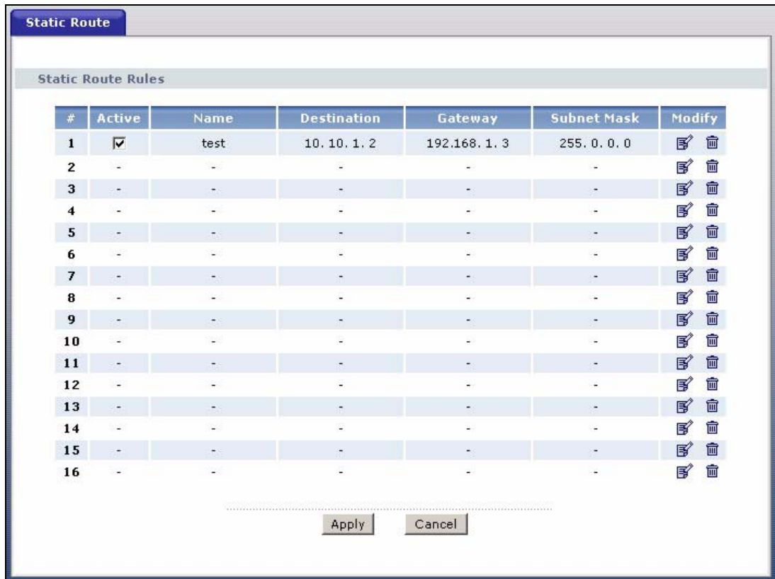
Figure 99 Static Route
