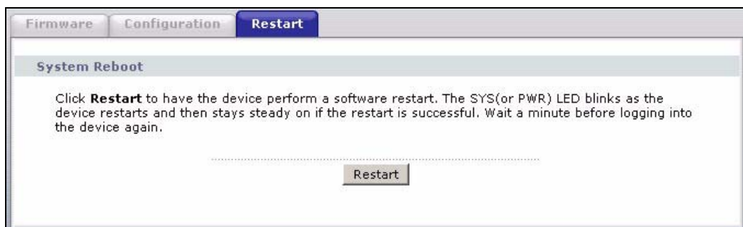
Figure 144 Restart Screen
