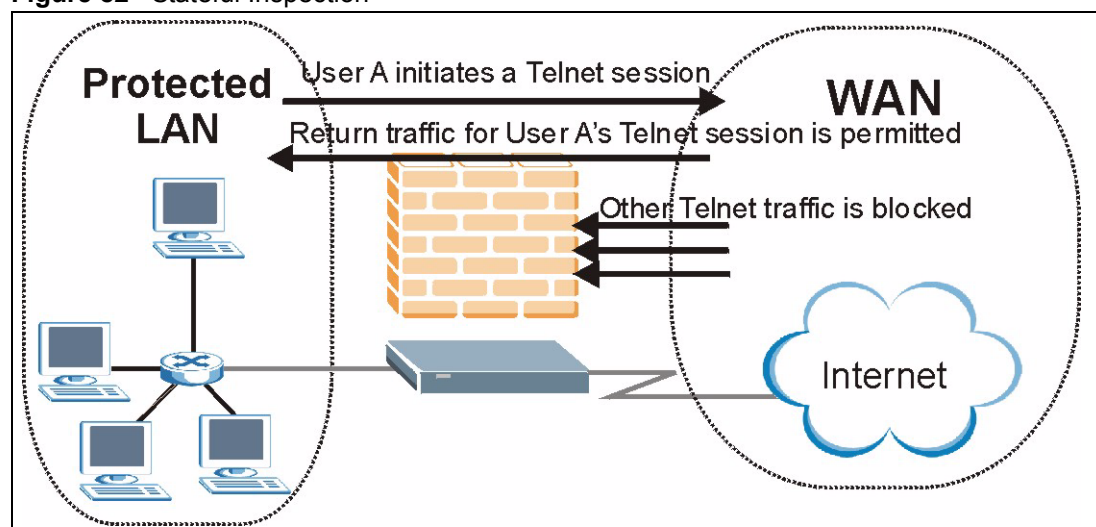
Figure 82 Stateful Inspection
