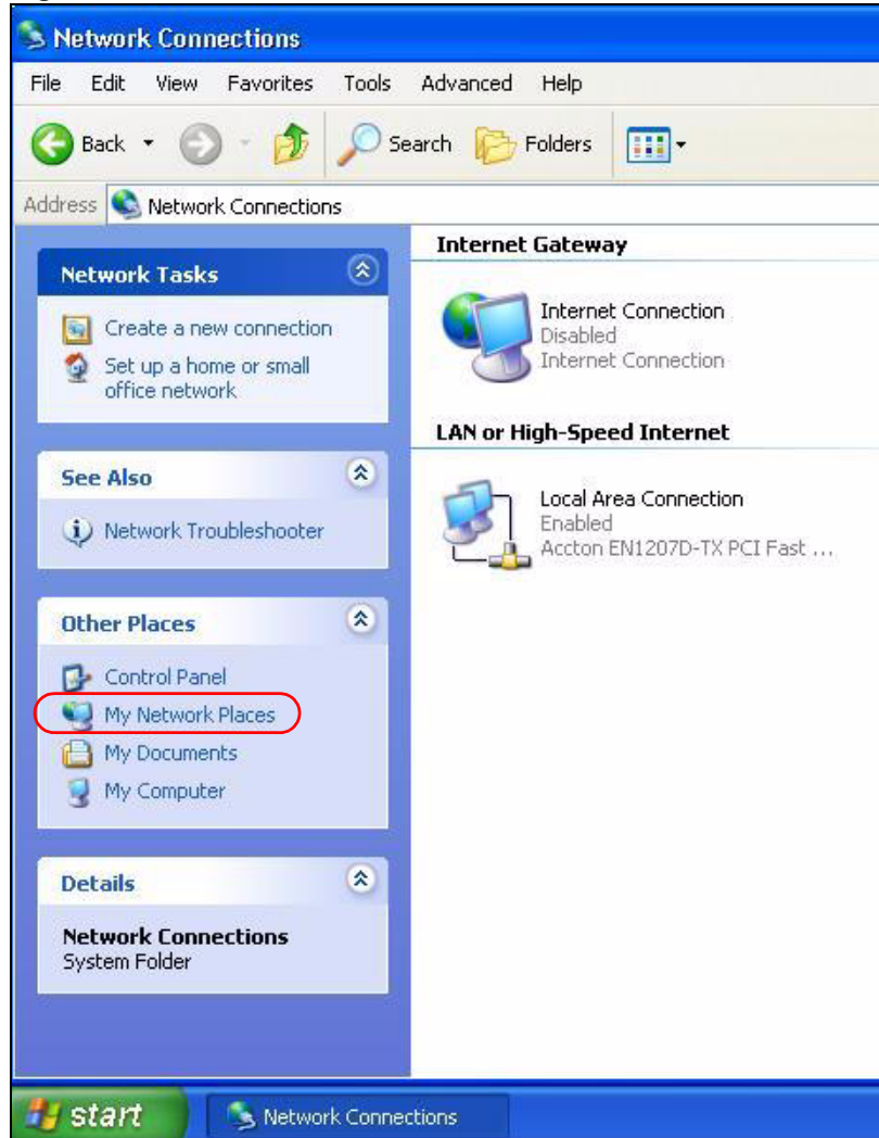
Figure 128 Network Connections
