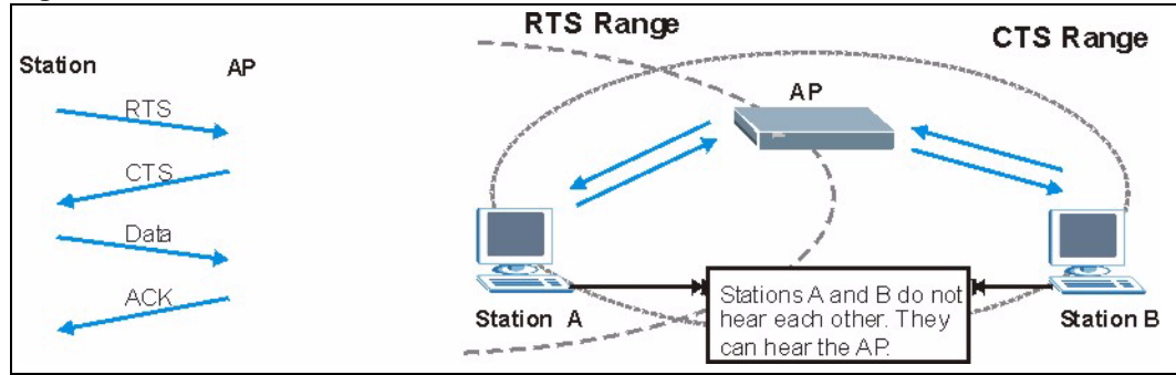
Figure 185 RTS/CTS
