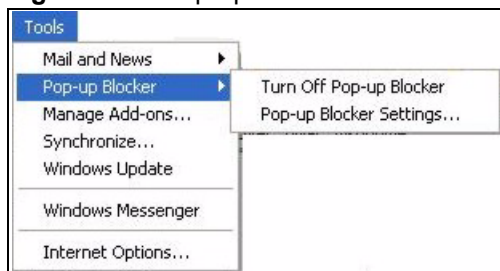
Figure 188 Pop-up Blocker
