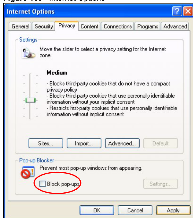
Figure 189 Internet Options
