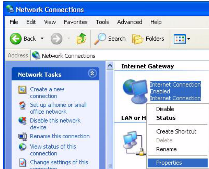
Figure 122 Network Connections
