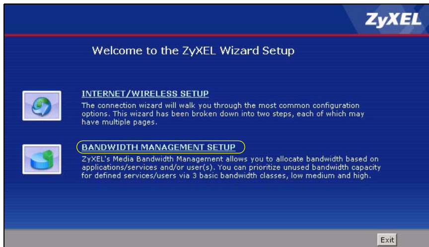
Figure 34 Wizard: Welcome
