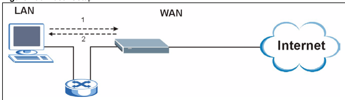
Figure 196 Ideal Setup
