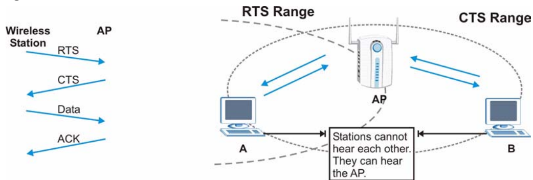
Figure 22 RTS/CTS
