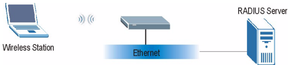
Figure 26 EAP Authentication
