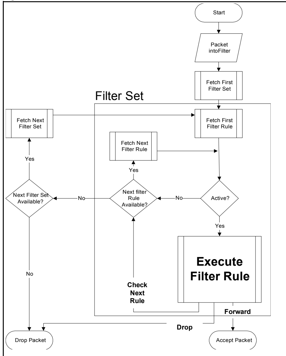
Figure 186 Filter Rule Process
