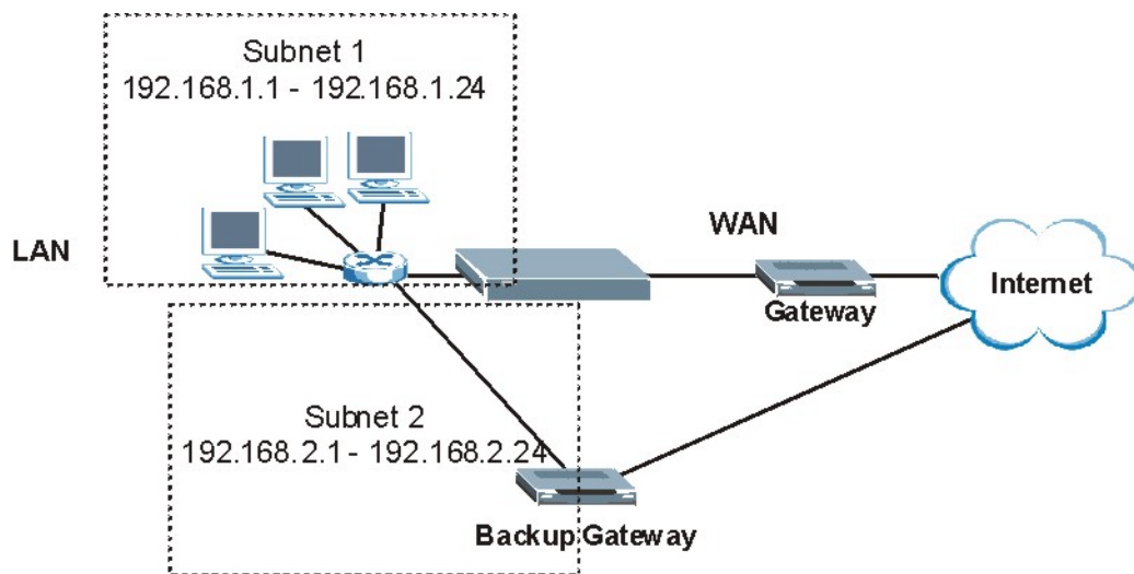
Figure 38 Traffic Redirect LAN Setup
