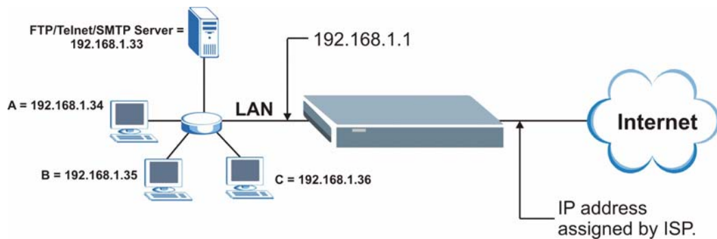
Figure 42 Multiple Servers Behind NAT Example
