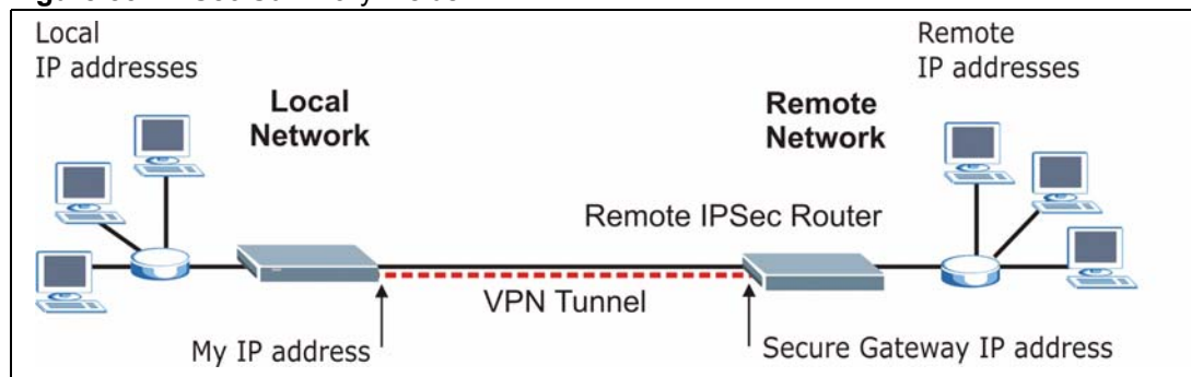
Figure 85 IPSec Summary Fields
