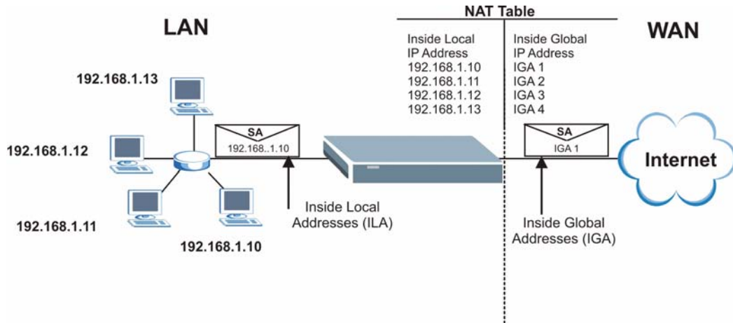
Figure 40 How NAT Works
