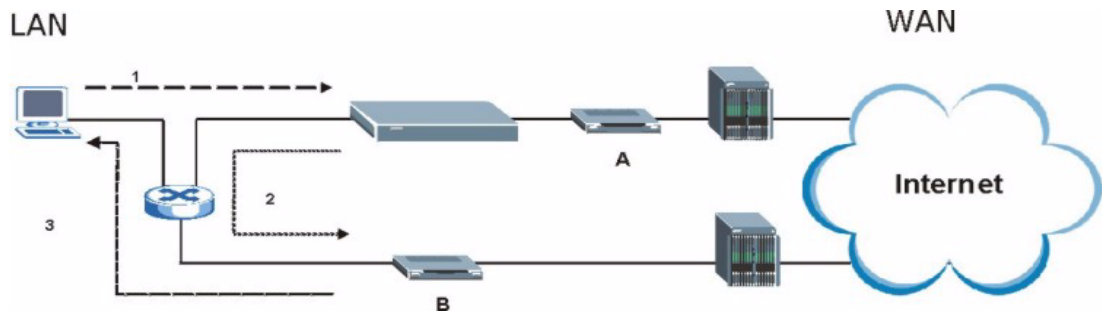
Figure 285 “Triangle Route” Problem
