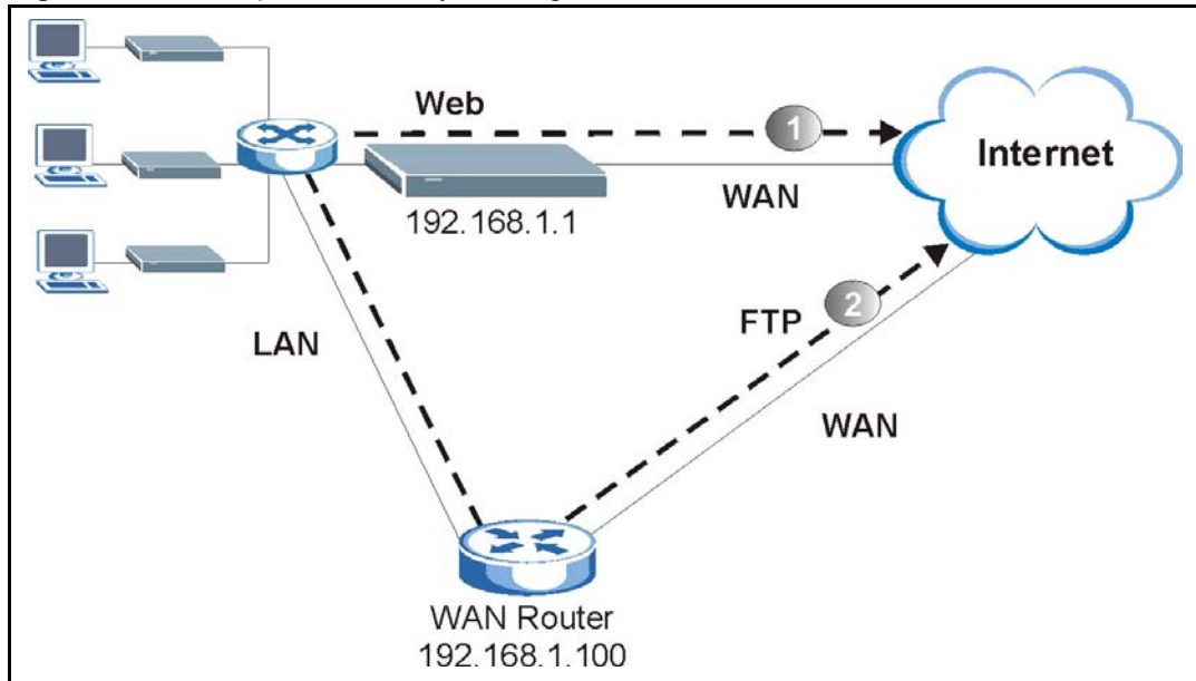
Figure 250 Example of IP Policy Routing
