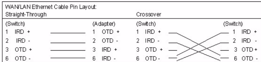
Figure 264 Ethernet Cable Pin Assignments
