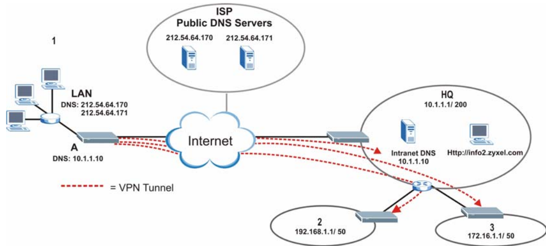
Figure 87 VPN Host using Intranet DNS Server Example
