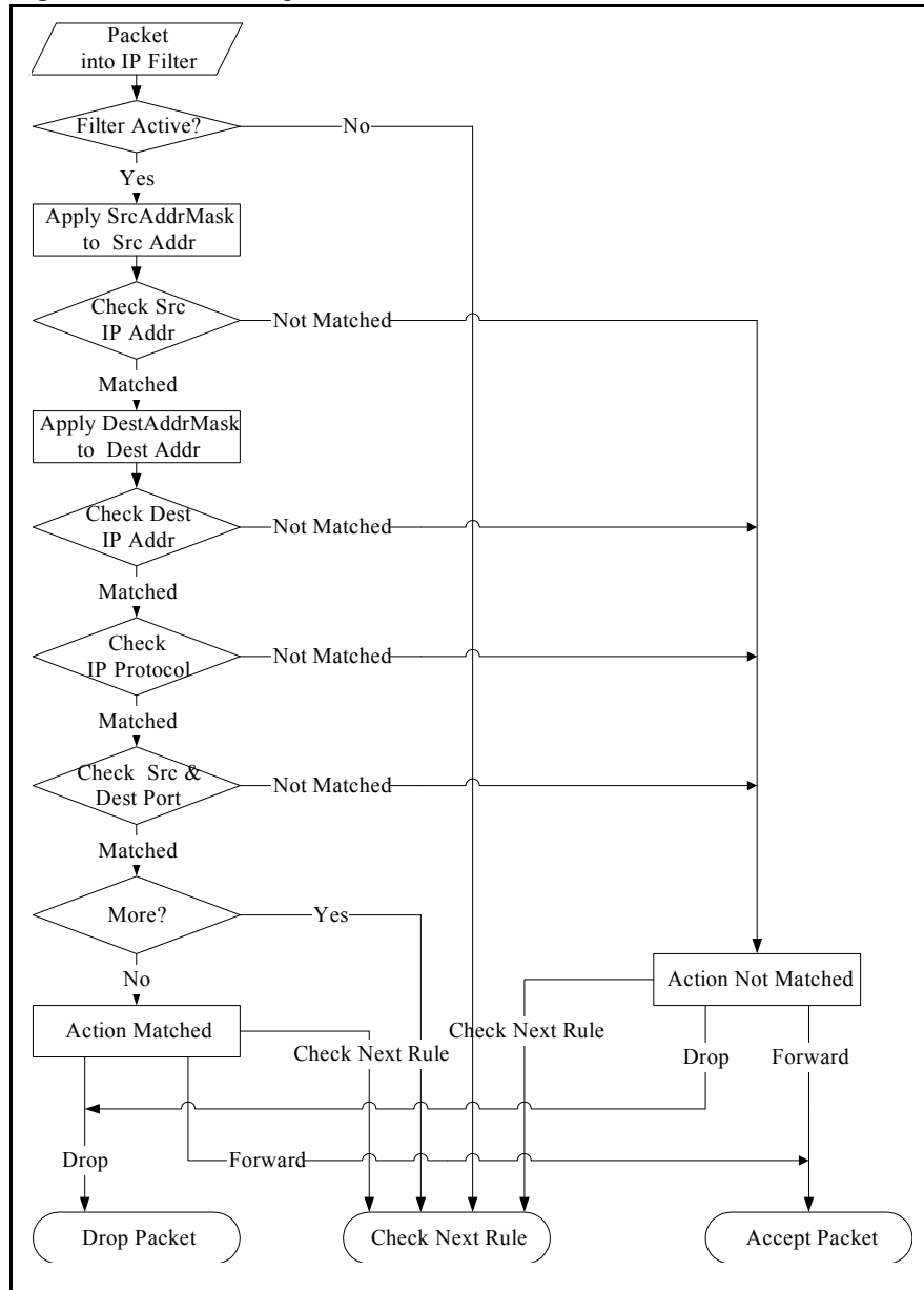
Figure 192 Executing an IP Filter
