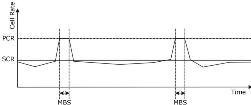
Figure 35 Example of Traffic Shaping
