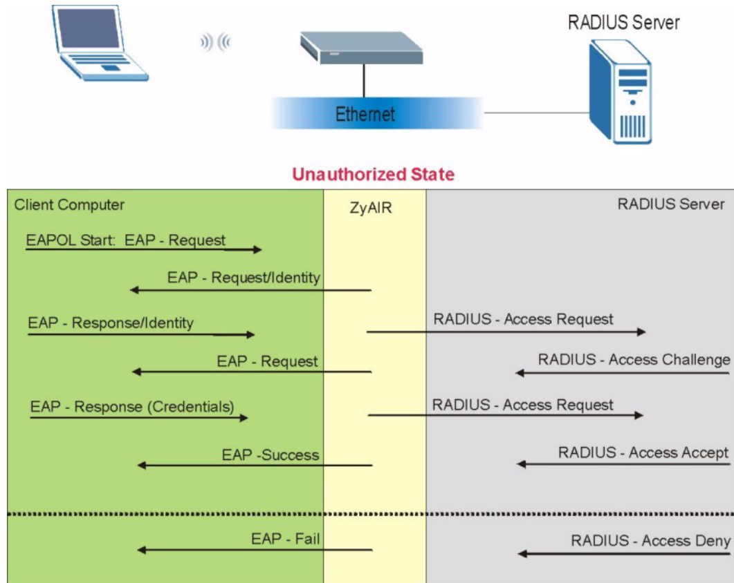
Figure 283 Sequences for EAP MD5–Challenge Authentication
