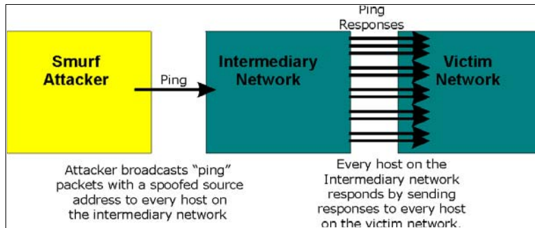
Figure 63 Smurf Attack
