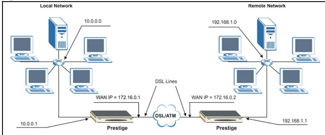
Figure 148 Sample IP Addresses for a TCP/IP LAN-to-LAN Connection
