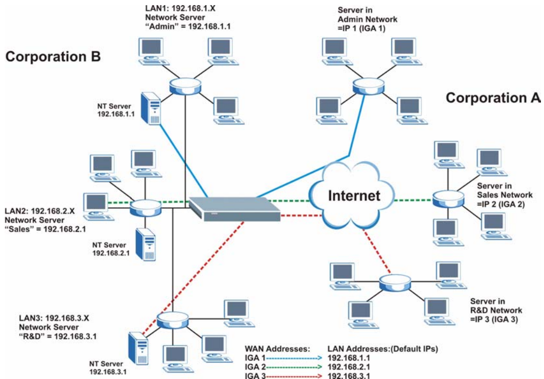
Figure 41 NAT Application With IP Alias
