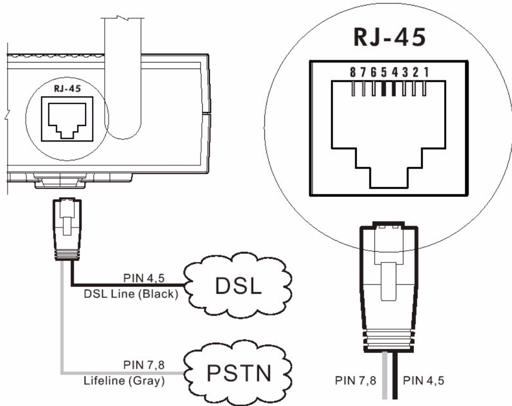
Figure 265 Prestige 2602HW-L DSL Port Pin Assignments
