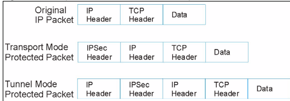
Figure 84 Transport and Tunnel Mode IPSec Encapsulation
