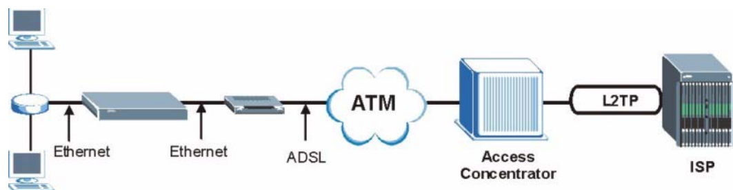
Figure 280 Prestige as a PPPoE Client
