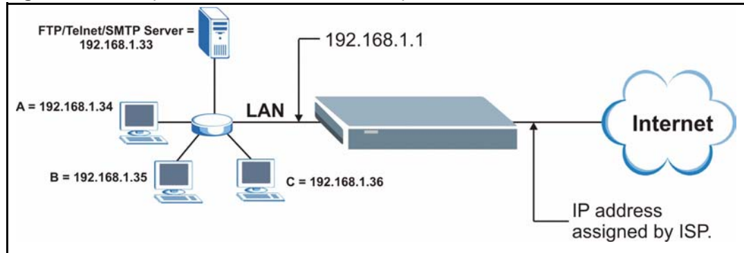
Figure 171 Multiple Servers Behind NAT Example
