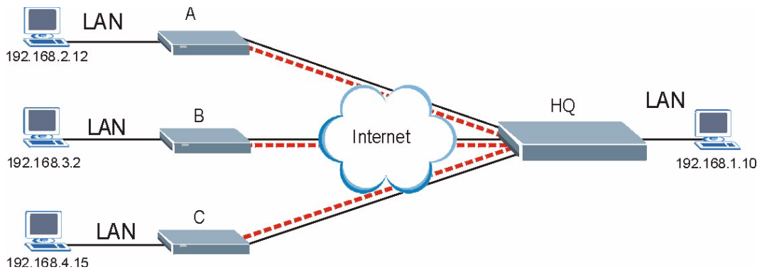
Figure 96 Telecommuters Using Unique VPN Rules Example
