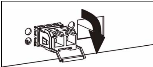
Figure 12 Opening the Transceiver's Latch Example
