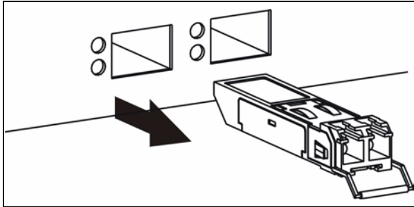
Figure 13 Transceiver Removal Example
