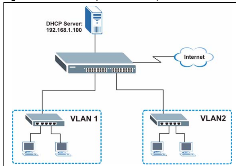
Figure 104 DHCP Relay Network Example
