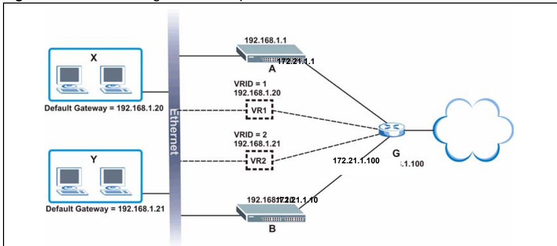
Figure 116 VRRP Configuration Example: Two Virtual Router Network
