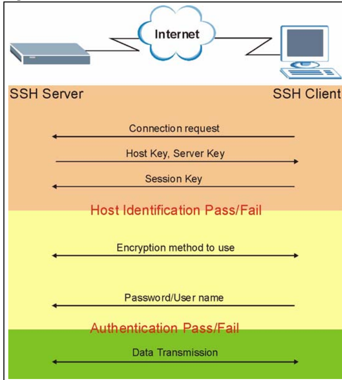
Figure 132 How SSH Works
