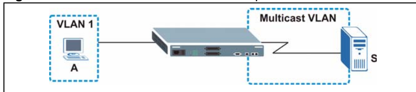
Figure 72 MVR Multicast Television Example
