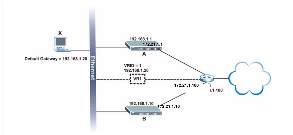
Figure 111 VRRP Configuration Example: One Virtual Router Network
