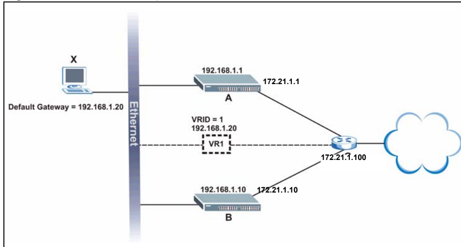
Figure 106 VRRP: Example 1
