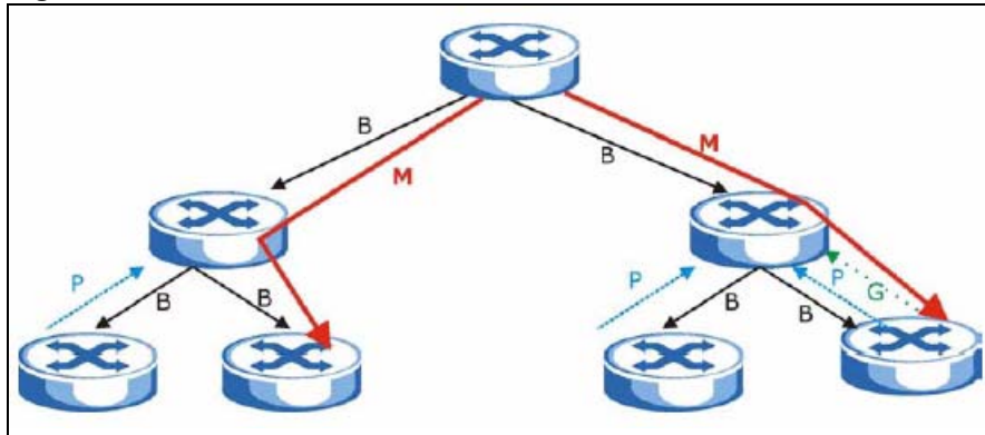
Figure 89 How DVMRP Works
