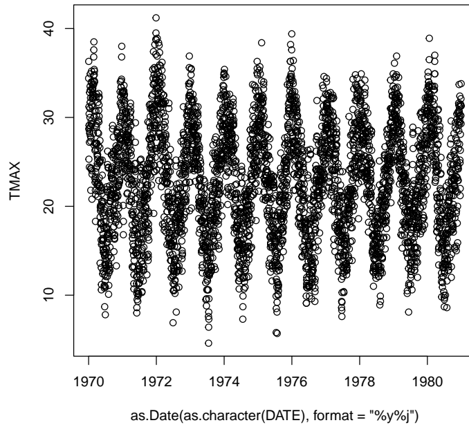
Figure 4: Daily maximum temperature series.
