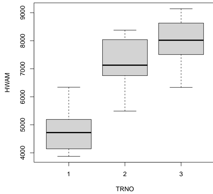
Figure 3: Yield box plot. Treatments; 1: without fertilization, 2: with 50kg/ha of urea, 3: with 100kg/ha of urea.
